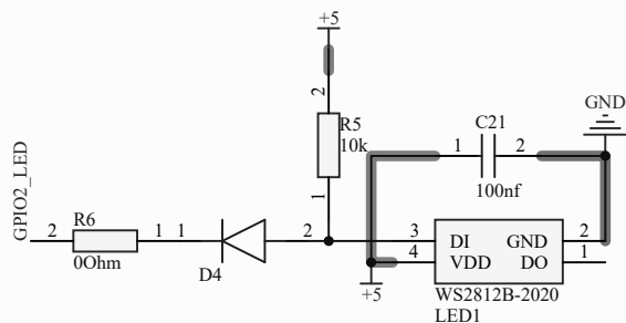
RGB LED
