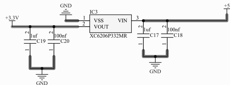
Voltage Regulator
