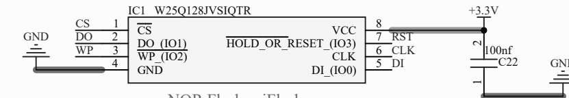
NOR Flash spiFlash
